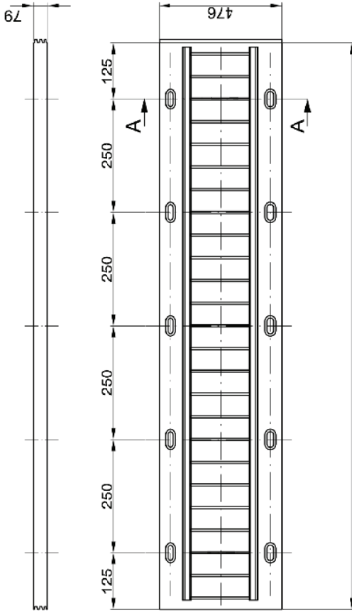
A-A ASSEMBLY DETAIL
